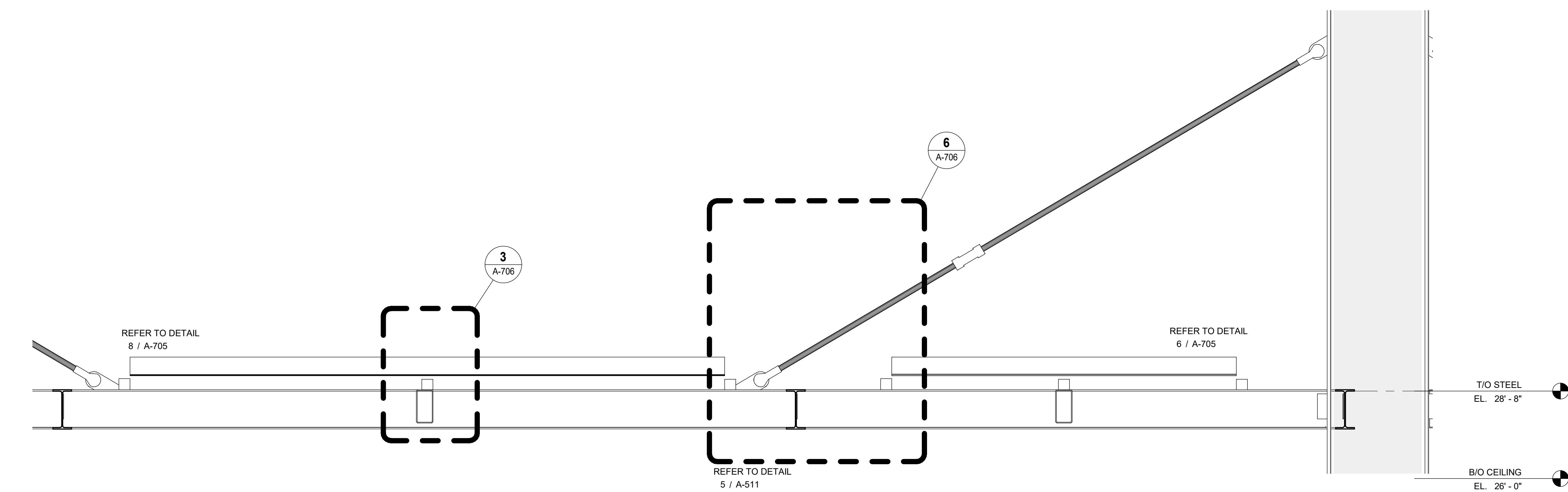
3 SECTION - ENLARGED PARTIAL SCALE: 1/2" = 1'-0"
