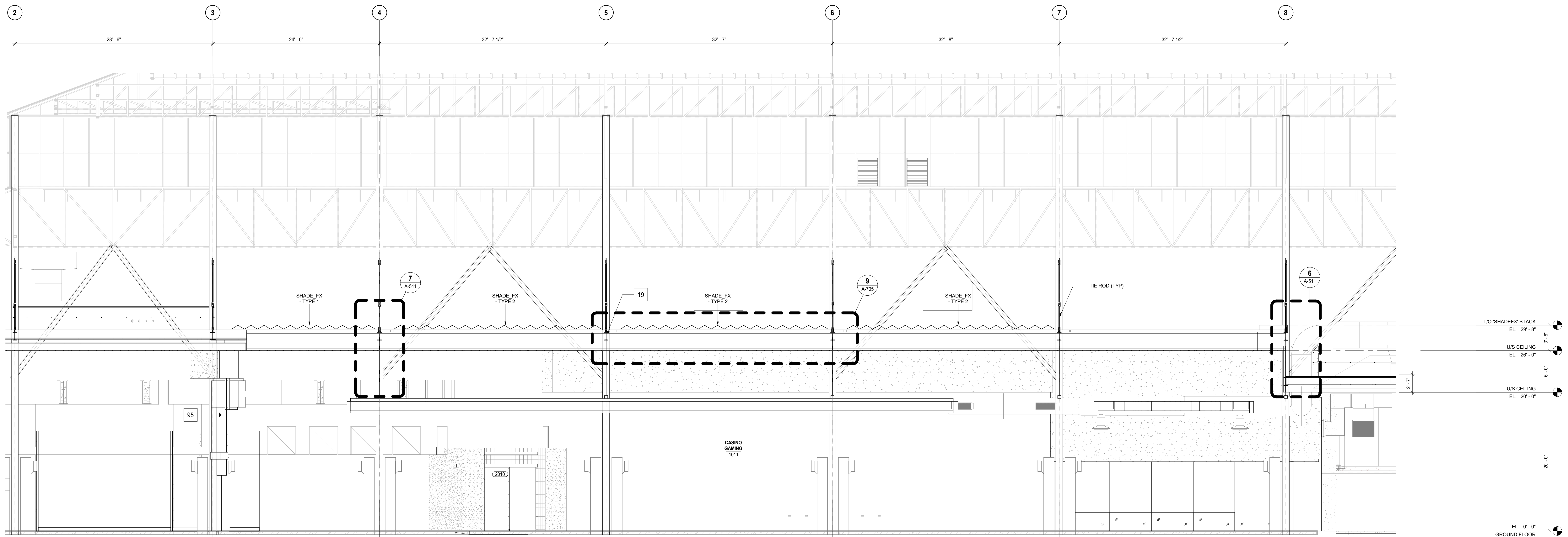
1 CEILING SECTION - CASINO AREA A SCALE: 3/16" = 1'-0"
