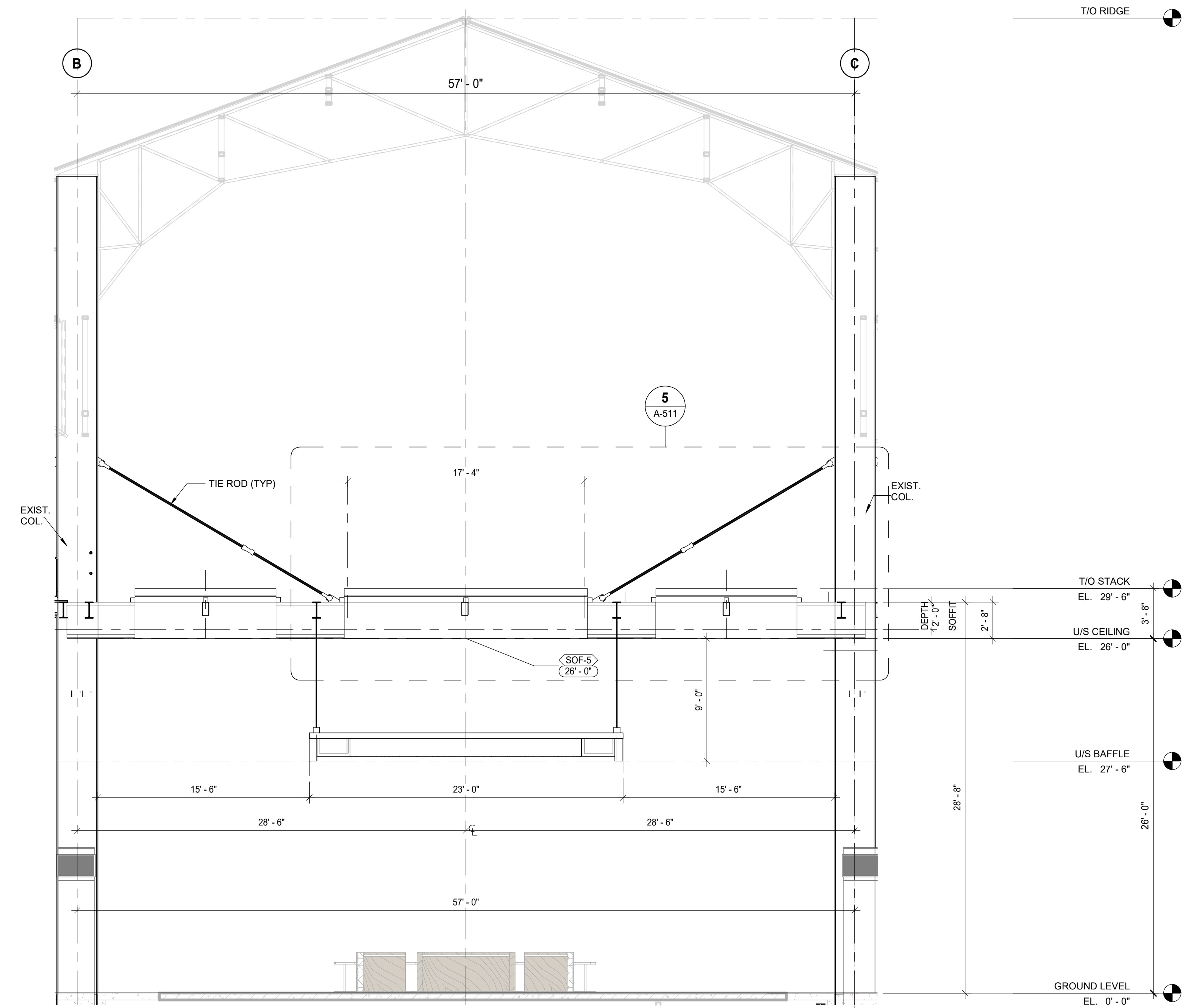
2 SECTION - ENLARGED SCALE: 3/16" = 1'-0"
